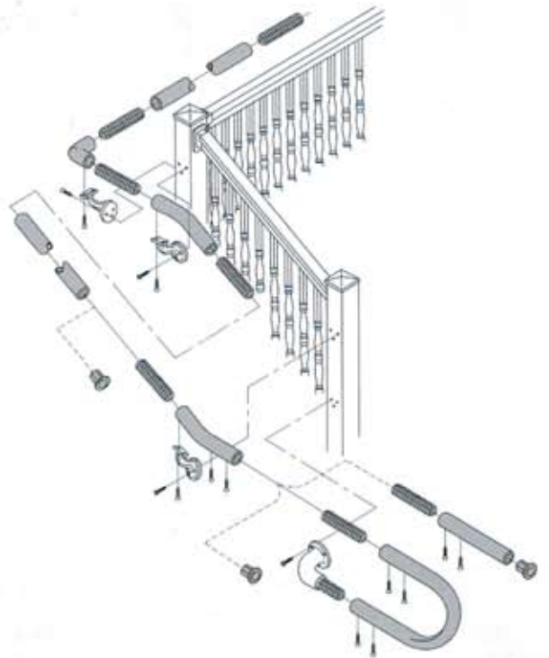
Corner Mounting Bracket LBGHRCBRKT
